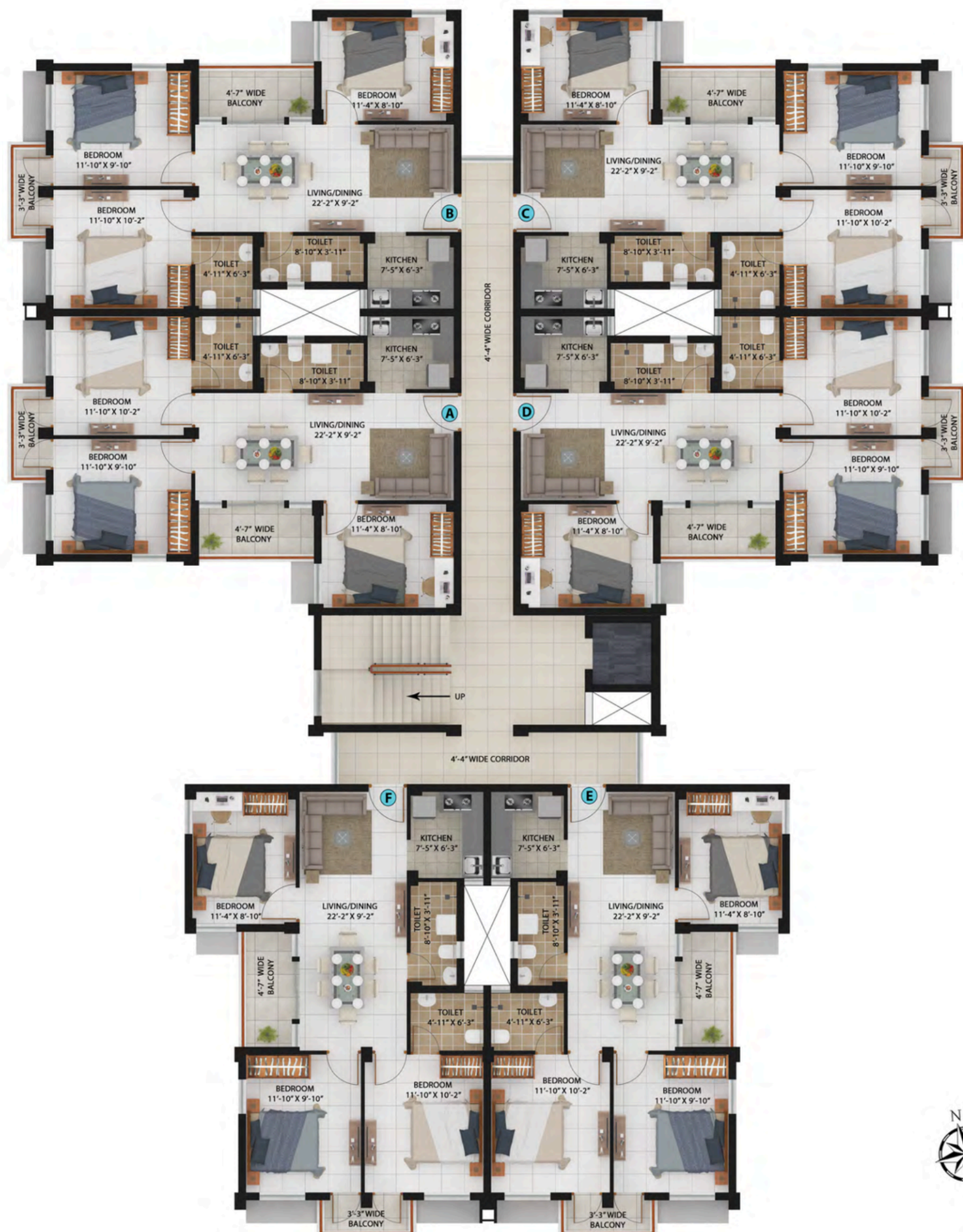
Block 1 | Typical floor plan (1st, 2nd, 3rd, 4th)
